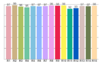
CRI: 96.9 (R1-R8)
