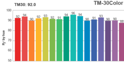
Color distortion
